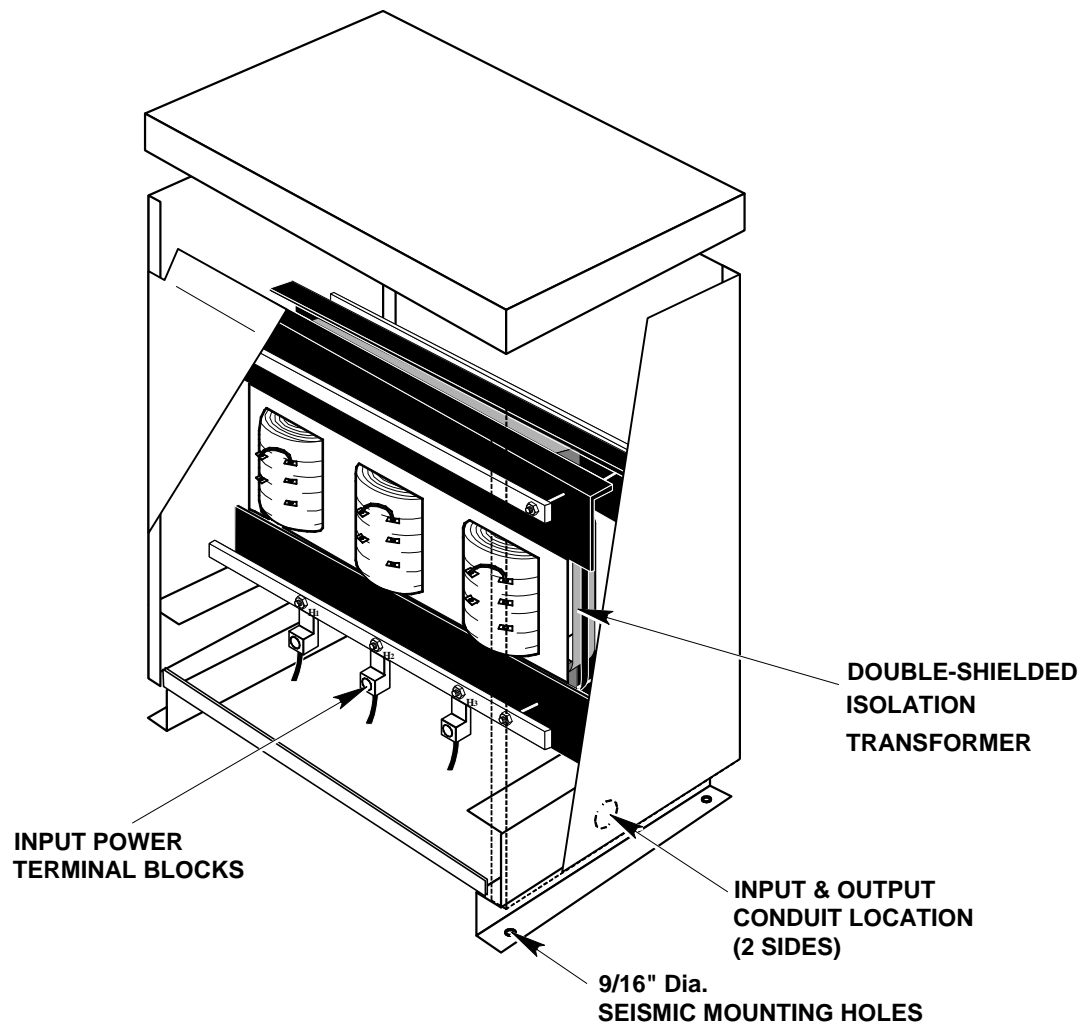
NRT FEATURES ILLUSTRATION 1-3
