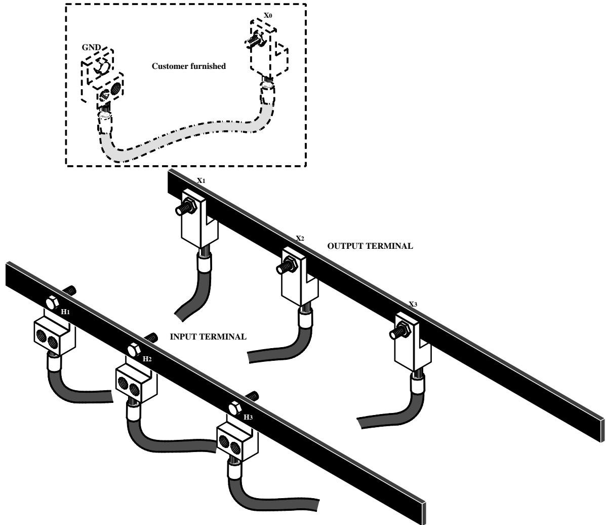
NRT INPUT & OUTPUT TERMINAL CONNECTION ILLUSTRATION 3-3
